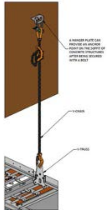
OFFIT BOLT-IN HANGER, PLATE DETAIL
