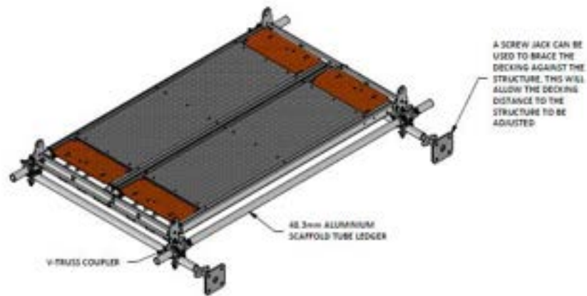
SCREW-JACK BRACING
