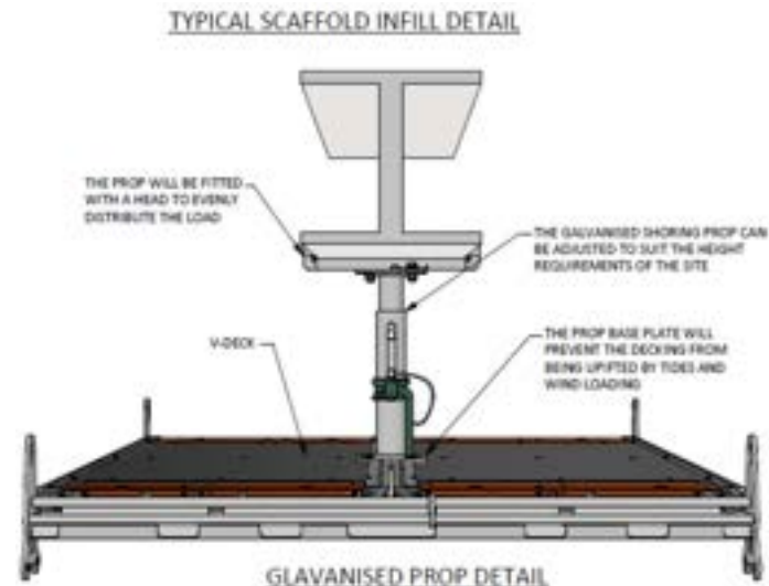
GALVANISED PROP DETAIL
